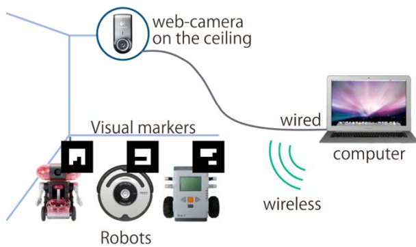
Figure 2 Example setup of the toolkit
